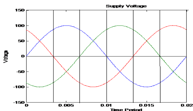
Fig 7: Three Phase Input Supply voltage Wave Form
