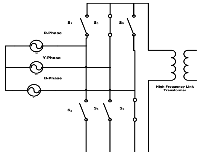
Fig 4: High Frequency Positive Conducting Cycle - Sector I
