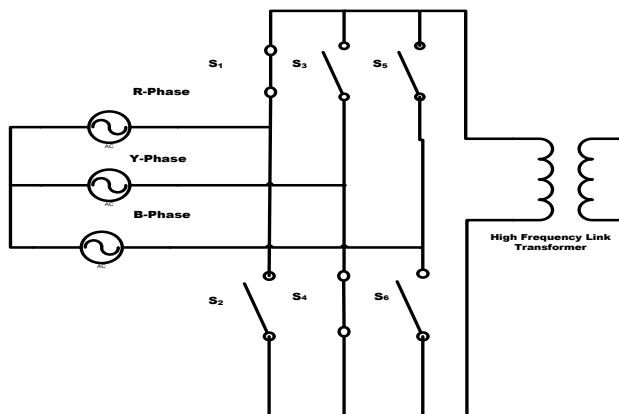
Fig. 5: High Frequency Negative Conducting Cycle- Sector I
