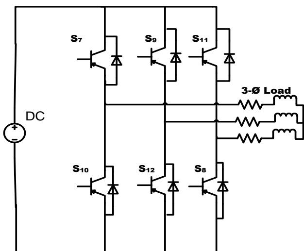
Fig 6: Circuit Diagram of Inversion
