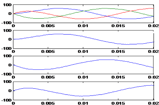
Fig 10: Output Current Waveforms
