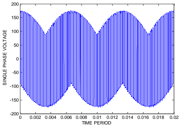
Fig 8: Single phase high frequency voltage waveform
