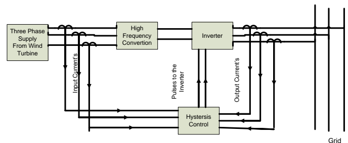
Fig 1: Block Diagram of Matrix Converter with Hysteresis Controller
