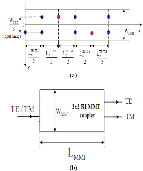
Fig. 6 Operating principle of the RI-MMI structure (a) graphical demonstration and (b) optical polarization splitter/combiner using a 2x2 RI-MMI coupler
