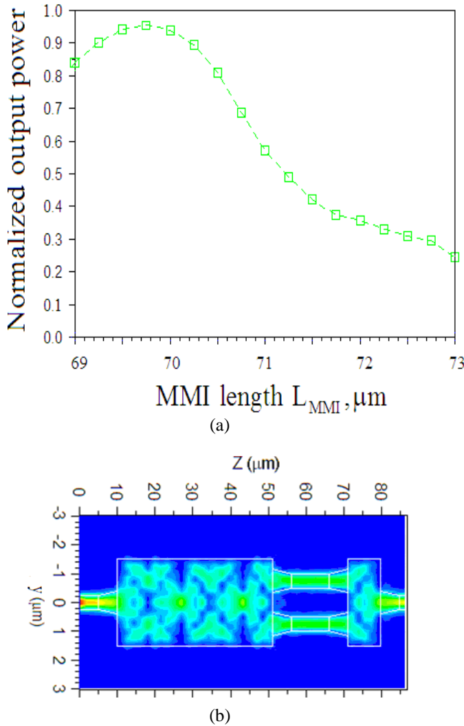
Fig. 5 (a) The normalized output powers of the TE mode filter at different lengths (b) the 3D-BPM simulation for the device having an optimised length of 69.7 \mu m and an input TE signal
