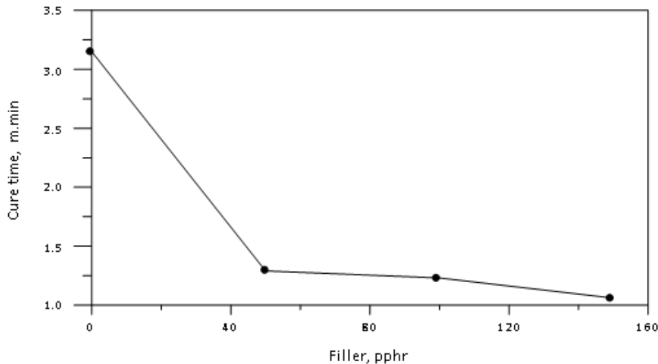
Fig. 3: Relation between the cure time and the shell powder percentage
