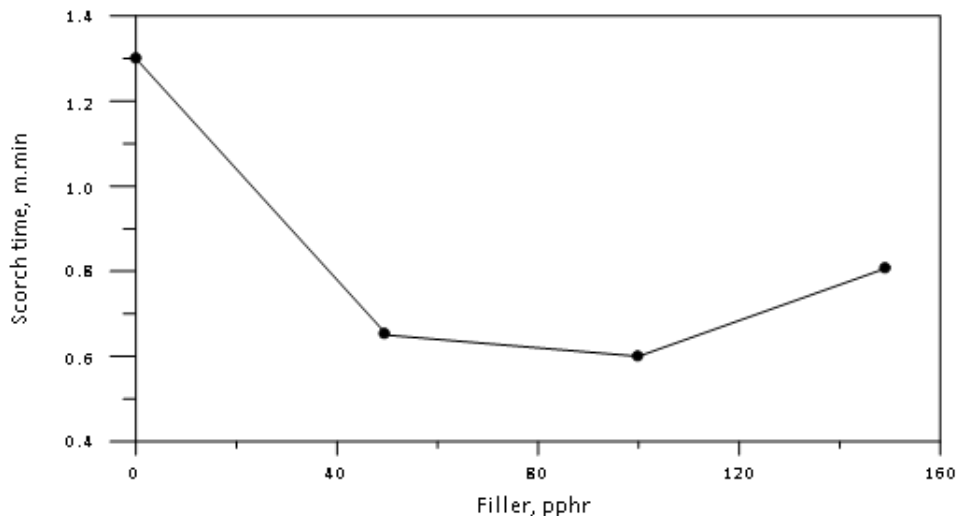
Fig. 2: Relation between the scorch time and the shell powder percentage
