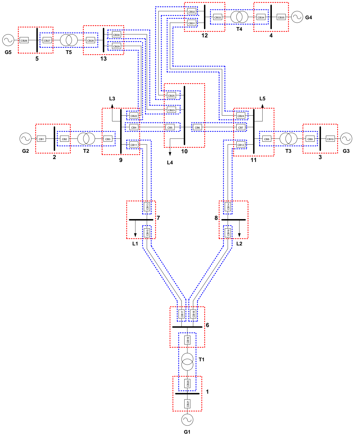
Fig. 3. The 13 bus system protection
