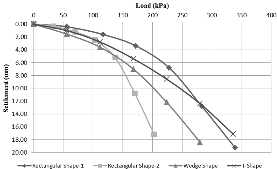
Fig. 8: Load-settlement curves for foundations prototypes on third modeled subsoil condition
