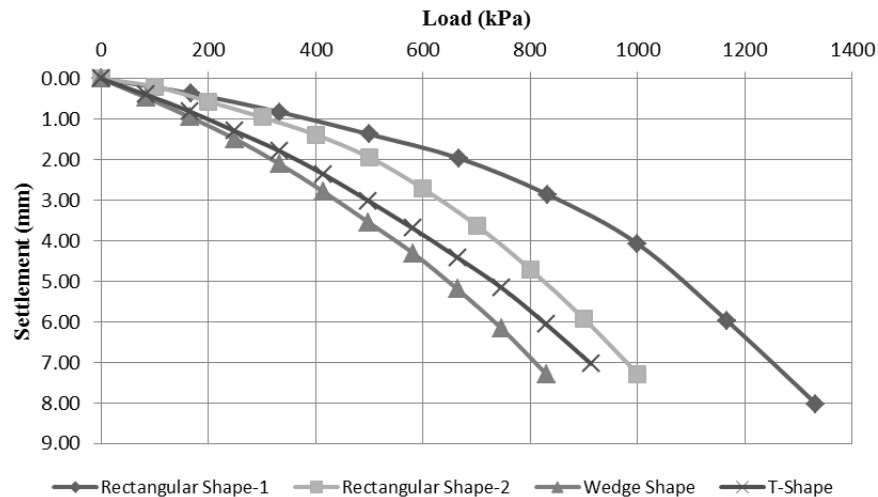
Fig. 6: Load-settlement curves for foundations prototypes on first modeled subsoil condition
