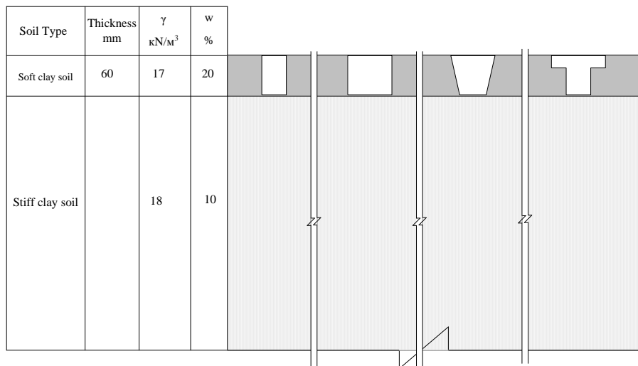
Fig. 4: Second modeled soil condition
