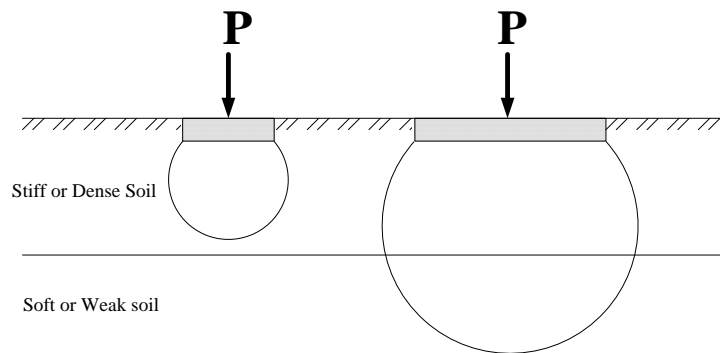
Fig. 9: Development of pressure bulbs under foundations with different widths
