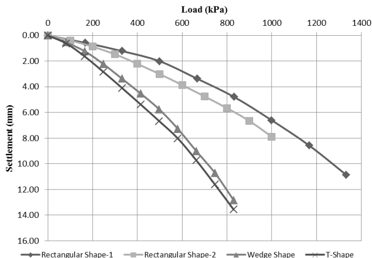
Fig. 7: Load-settlement curves for foundations prototypes on second modeled subsoil condition
