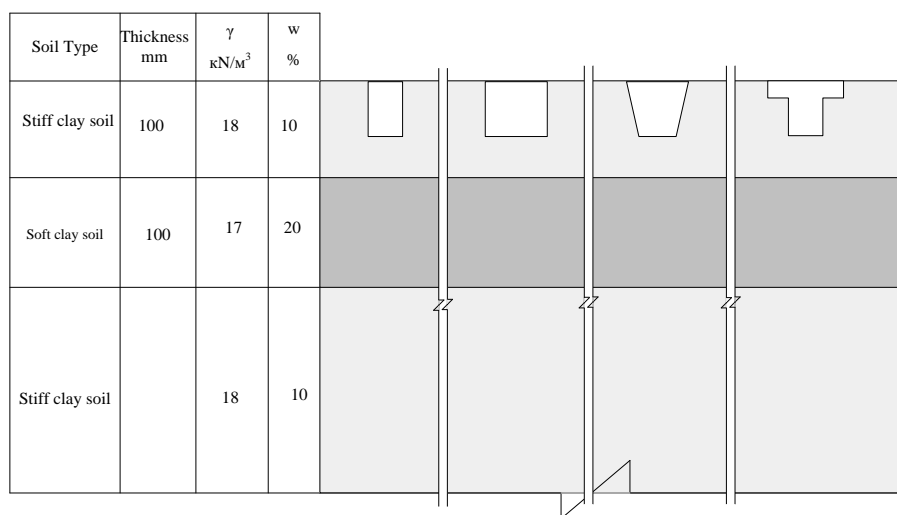
Fig. 5: Third modeled soil condition
