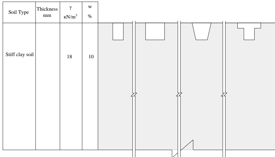
Fig. 3: First modeled soil condition
