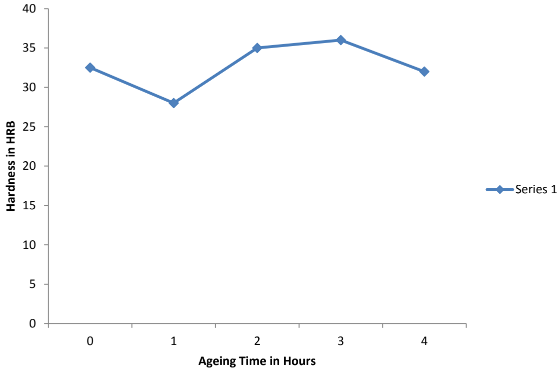
Figure 1: Effect of Ageing Time on the Hardness Values of 75Pb-15Sb-10Sn/ 10% v/v SiO 2 Particulate Composite.
