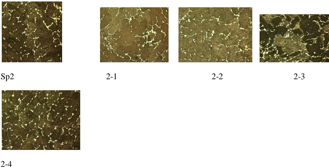
Plate 1: micrographs show the as cast sample (sp2), sample aged for 1hr (2-1), sample aged for 2hrs (2-2), sample aged for 3hrs (2-3), and sample aged for 4hrs (2-4) (etched using 2% Nital solution) x500
