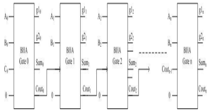
Figure 10. N-bit Ripple Carry Adder
