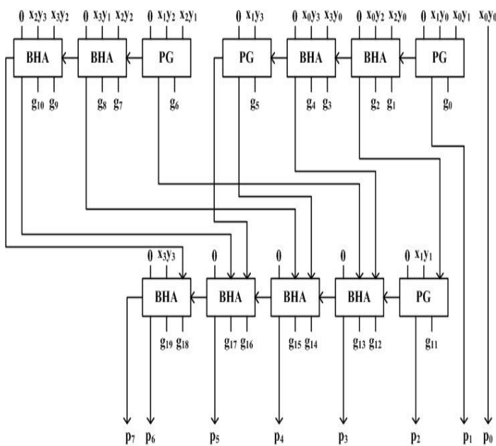
Figure 12. Proposed architecture for 4x4 Reversible multiplier using BHA and PERES Gate.
