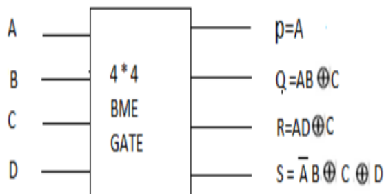
Figure 8: BME gate
