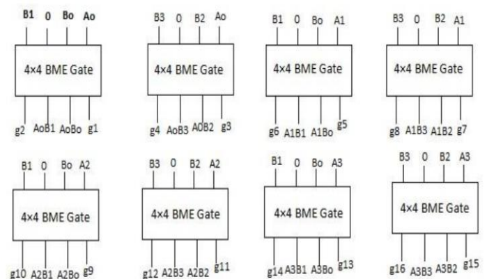
Figure 11: Partial Product Generation using BME Gate.
