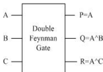
Figure 4. Double Feynman Gate
