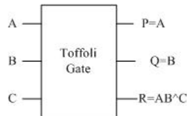
Figure 5. TOFFOLI Gate
