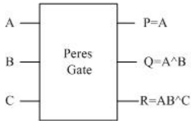
Figure 7. PERES Gate
