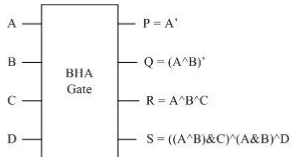
Figure 9. BHA gate
