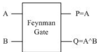
Figure 3. FEYMAN Gate
